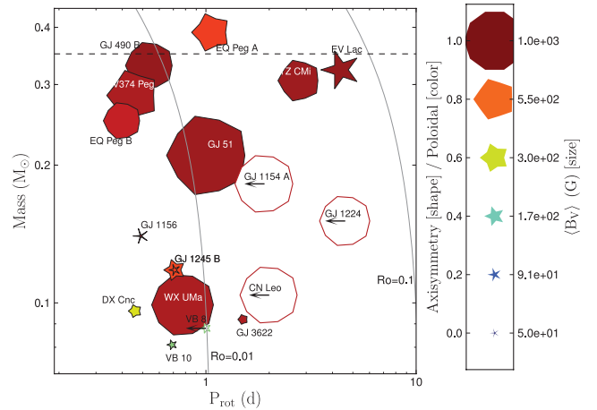
Figure 1. Mass–period diagram of fully-convective stars derived from spectropolarimetric data and ZDI by Morin et al. (2008b), Phan-Bao et al. (2009) and M10a. The symbol size represents the reconstructed magnetic energy, the colour ranges from blue to red for purely toroidal to purely poloidal field, and the shape depicts the degree of axisymmetry from a sharp star for non-axisymmetric to a regular decagon for axisymmetric. For a few stars of the sample, M10a could not perform a definite ZDI reconstruction; in these cases, only an upper limit of the rotation period is known and the magnetic flux is extrapolated; those objects are depicted as the empty symbols. The theoretical fully-convective limit is depicted as the horizontal dashed line. The thin solid lines represent contours of constant Rossby number Ro = 0.01 (left-hand side) and 0.1 (right-hand side), as estimated in M10a.
