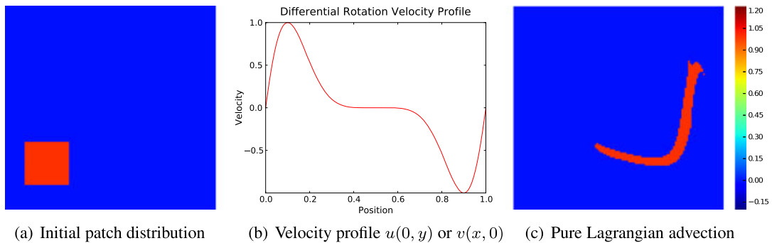
Figure 5. (a) Initial condition (intial patch distribution), (b) velocity profile [ u(0, y) or v(x, 0) ], and (c) final distribution (pure Lagragnian advection) for the two-dimensional advection test case.
