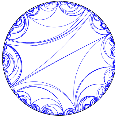
Figure 9: A sample of \mathcal{H} .
