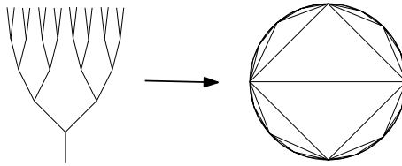
Figure 7: A binary tree full up to level 5 and its lamination limit.
