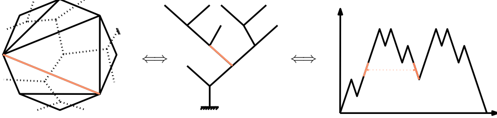
Figure 3: Duality with trees and excursion.
